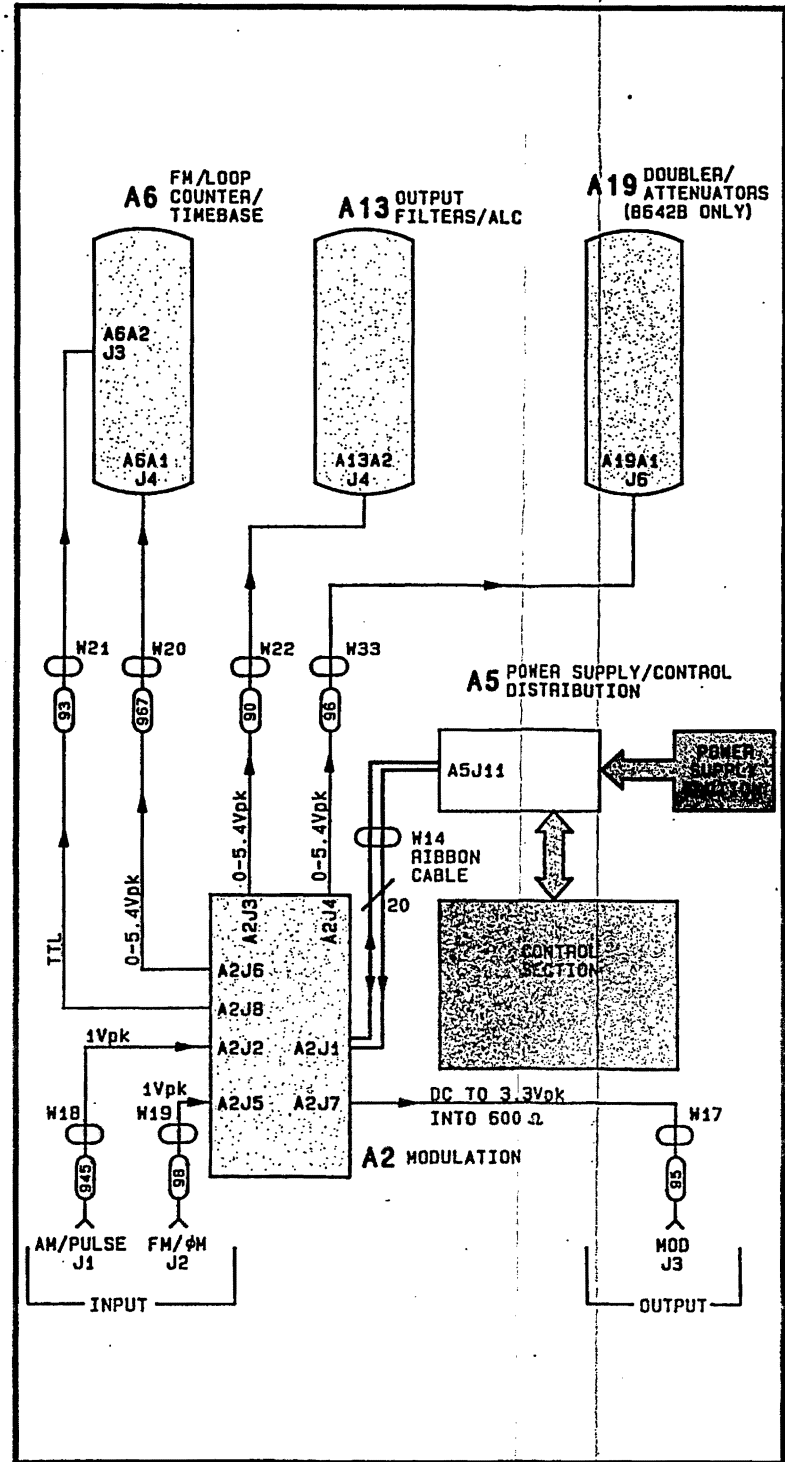
Figure 3E-100. A2 Modulation Module Diagnostics.
