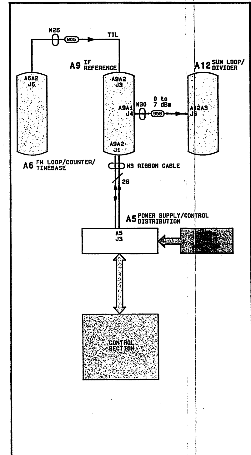
Figure 3H-100. A9 IF Reference Module Diagnostics.
