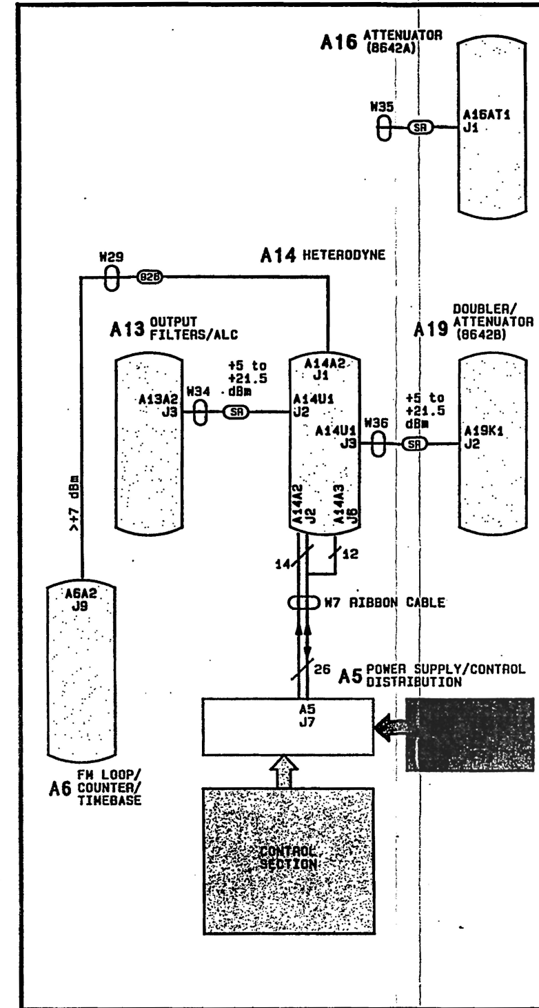
Figure 3L-100. A14 Heterodyne Module Diagnostics.
