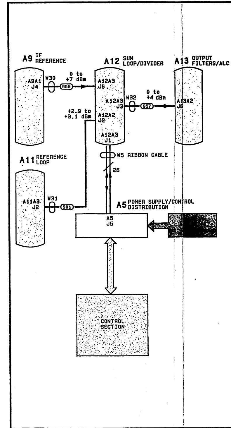
Figure 3J-100. A12 Sum Loop/Divider Module Diagnostics.
