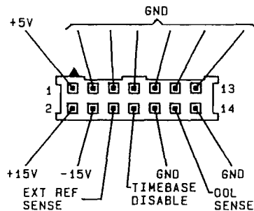
Figure 3F-2. Cable Plug W1P3 Signal Locator
