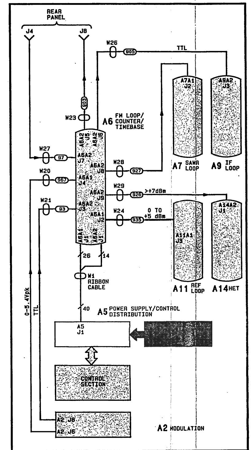
Figure 3F-100. A6 FM Loop/Counter/Timebase Module Diagnostics.
